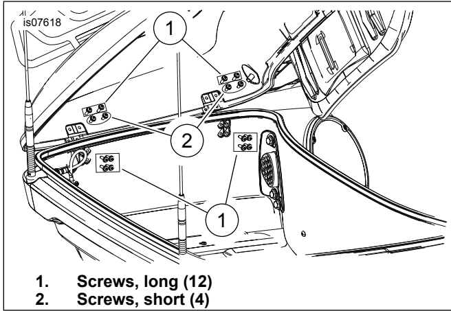
Figure 3. Replace Hinges
