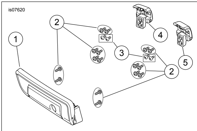
Figure 4. Service Parts: Latch Handle and Hinge Kit
