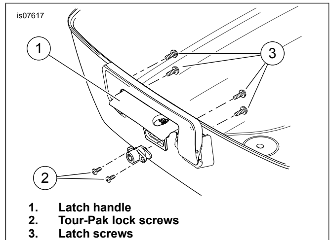
Figure 2. Latch Handle and Lockset Assembly
