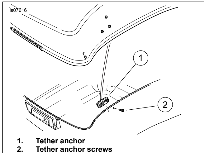
Figure 1. Tether Anchor Screws
