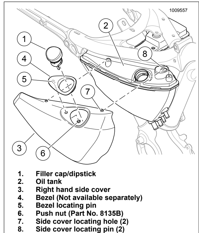
Figure 1. Right Hand Side Cover Installation
