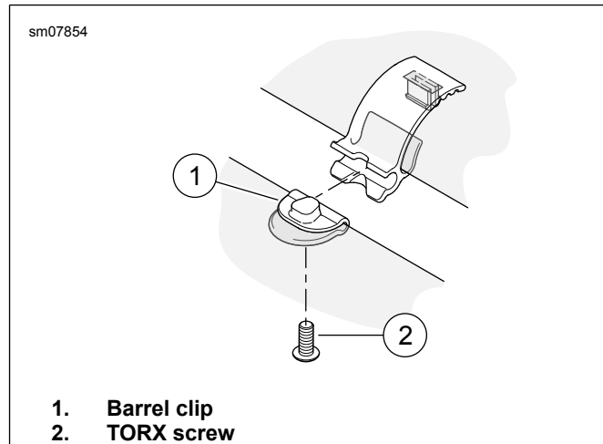
Figure 3. Barrel Clip
