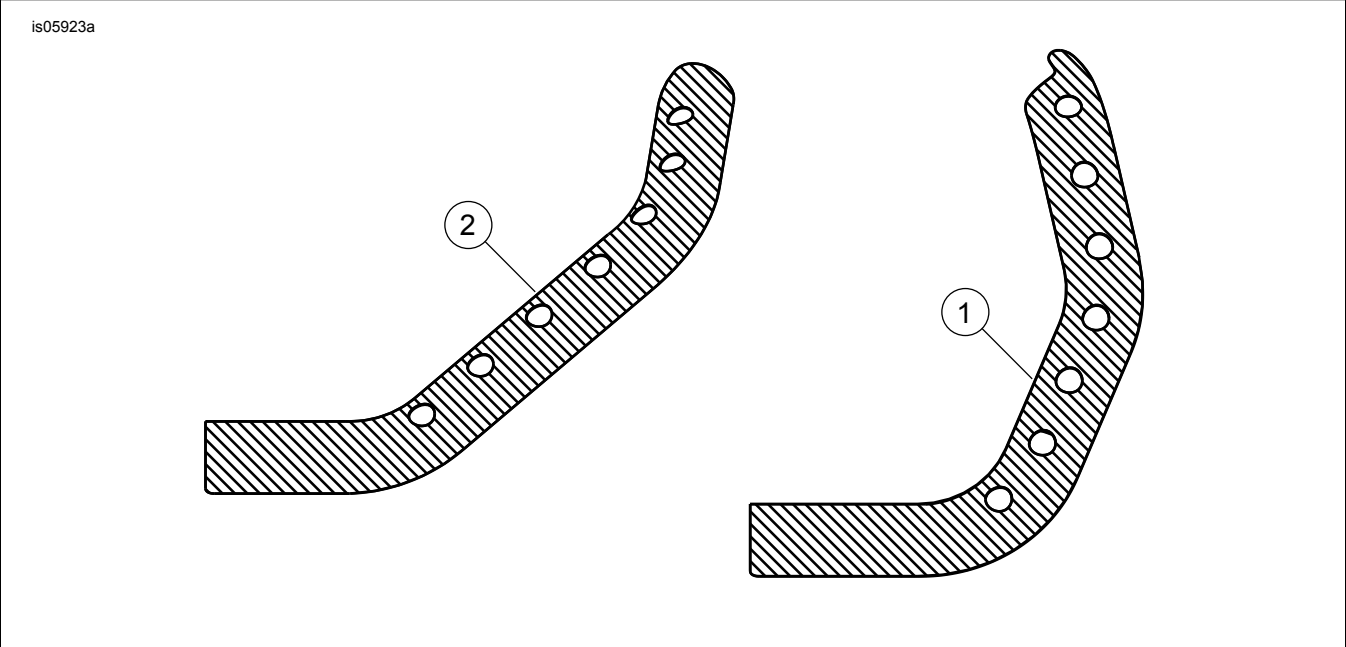
Figure 2. Service Parts: Sportster Exhaust Heat Shields
