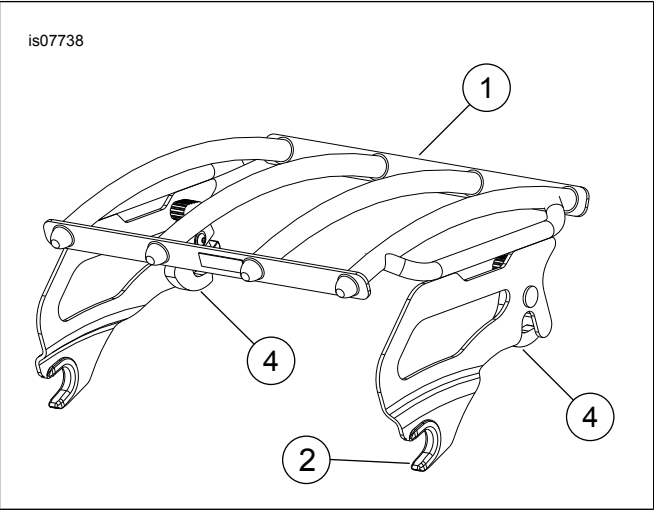
Figure 4. Service Parts: Detachable Solo Luggage Rack
