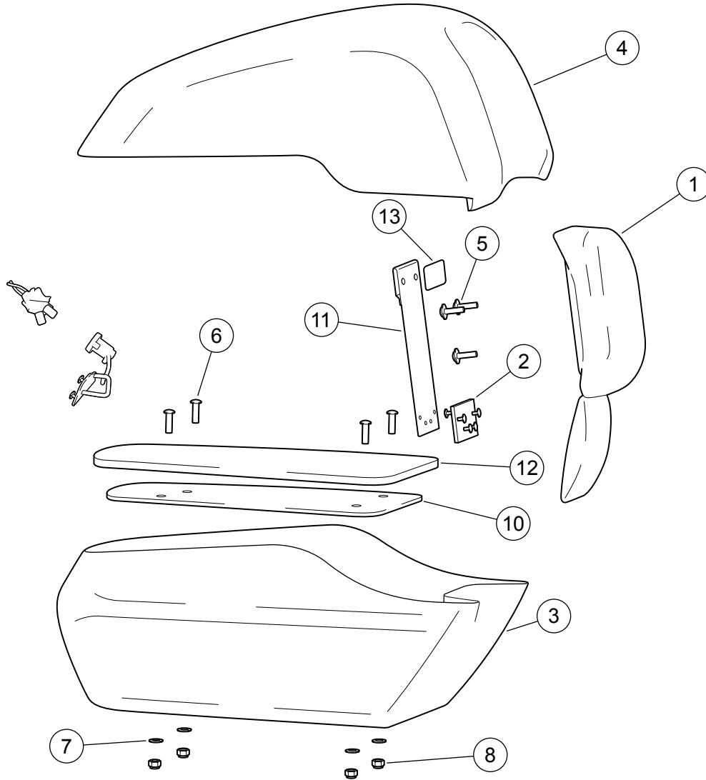
Figure 1. Service Parts: Leather Tour-Pak (Typical)
