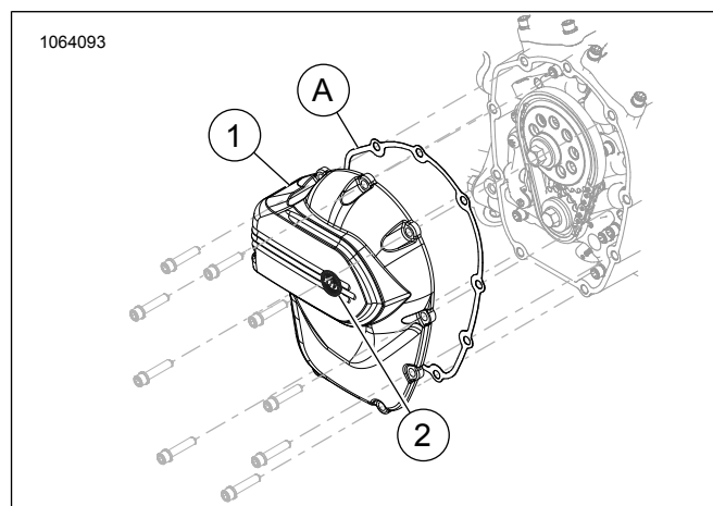
Figure 1. Milwaukee-Eight Cam Cover
