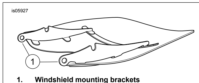
1. Windshield mounting brackets Figure 4. Windshield Mounting Brackets
