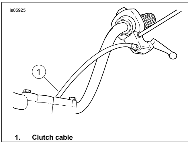
1. Clutch cable Figure 2. New Clutch Cable Routing
