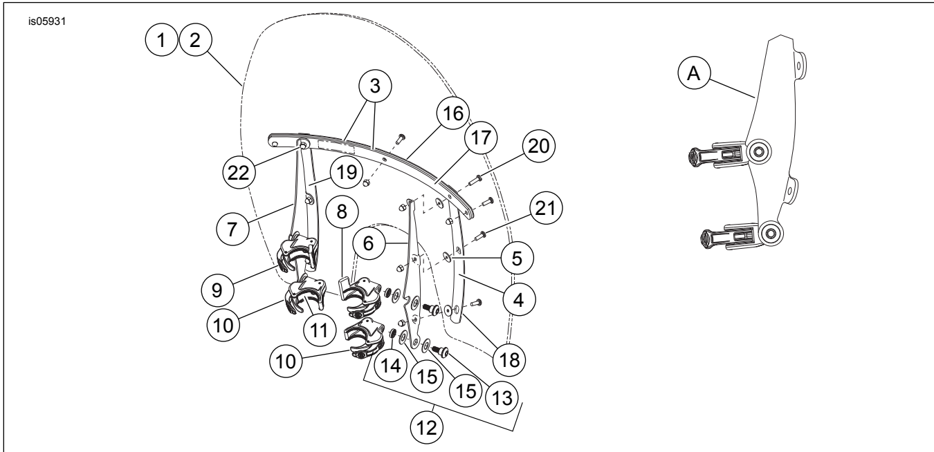
Figure 6. Service Parts: Quick Release Detachable Windshield Kits
