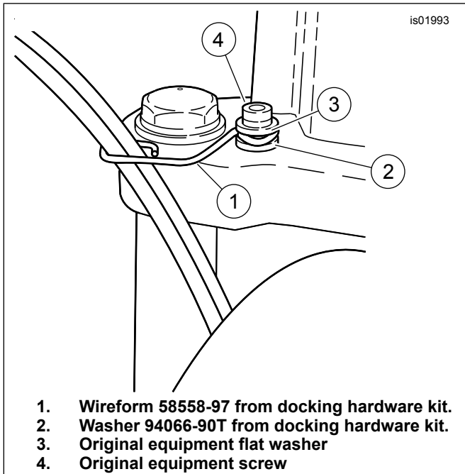
Figure 1. Throttle Cable Attachment
