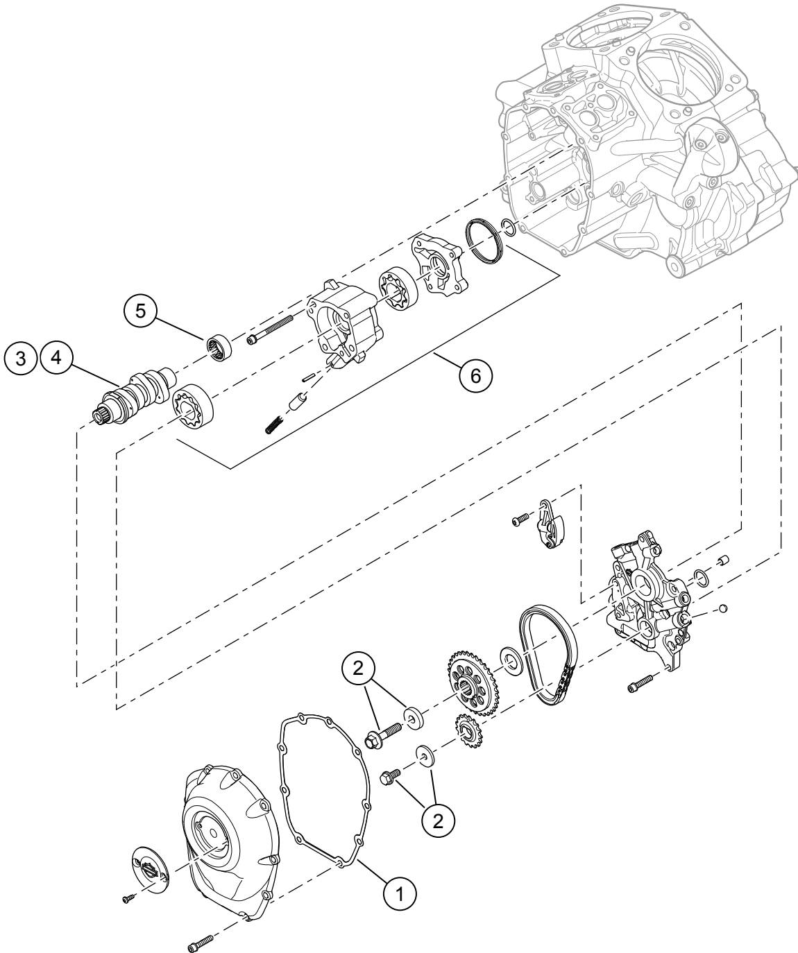
Figure 4. Mga Pamalit na Piyesa: Screamin' Eagle Milwaukee-eight Stage 2 Kit
