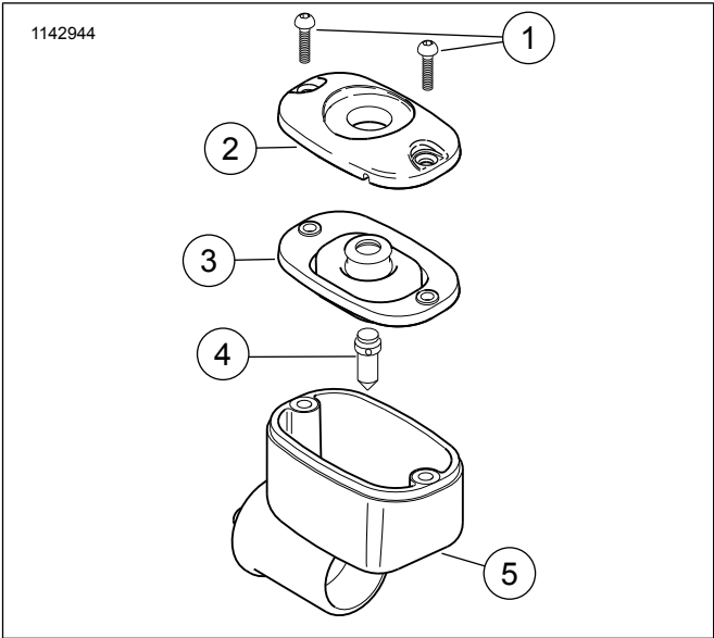
Figure 1. Service Parts: Master Cylinder Cover Kits
