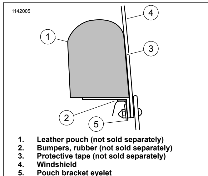
Figure 2. Fairing Clip Attachment, Side View
