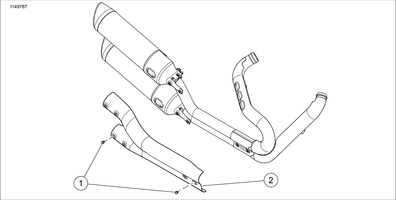
Figure 1. Service Parts: Dyna Model Exhaust Shields
