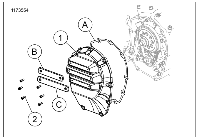
Figure 1. Milwaukee-Eight Cam Cover (Typical)
