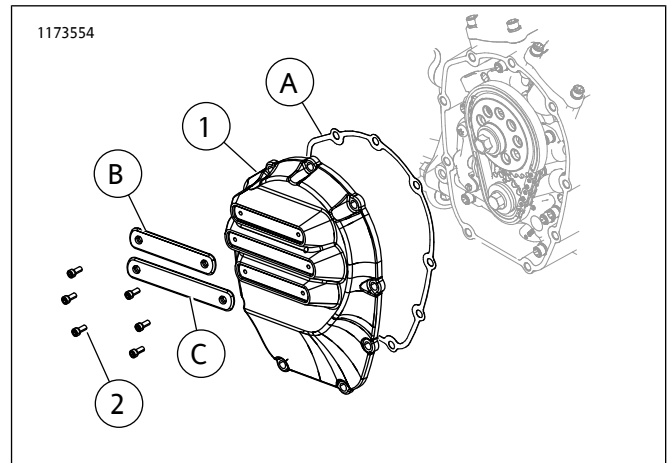
图1. Milwaukee-Eight 凸轮盖(典型)
