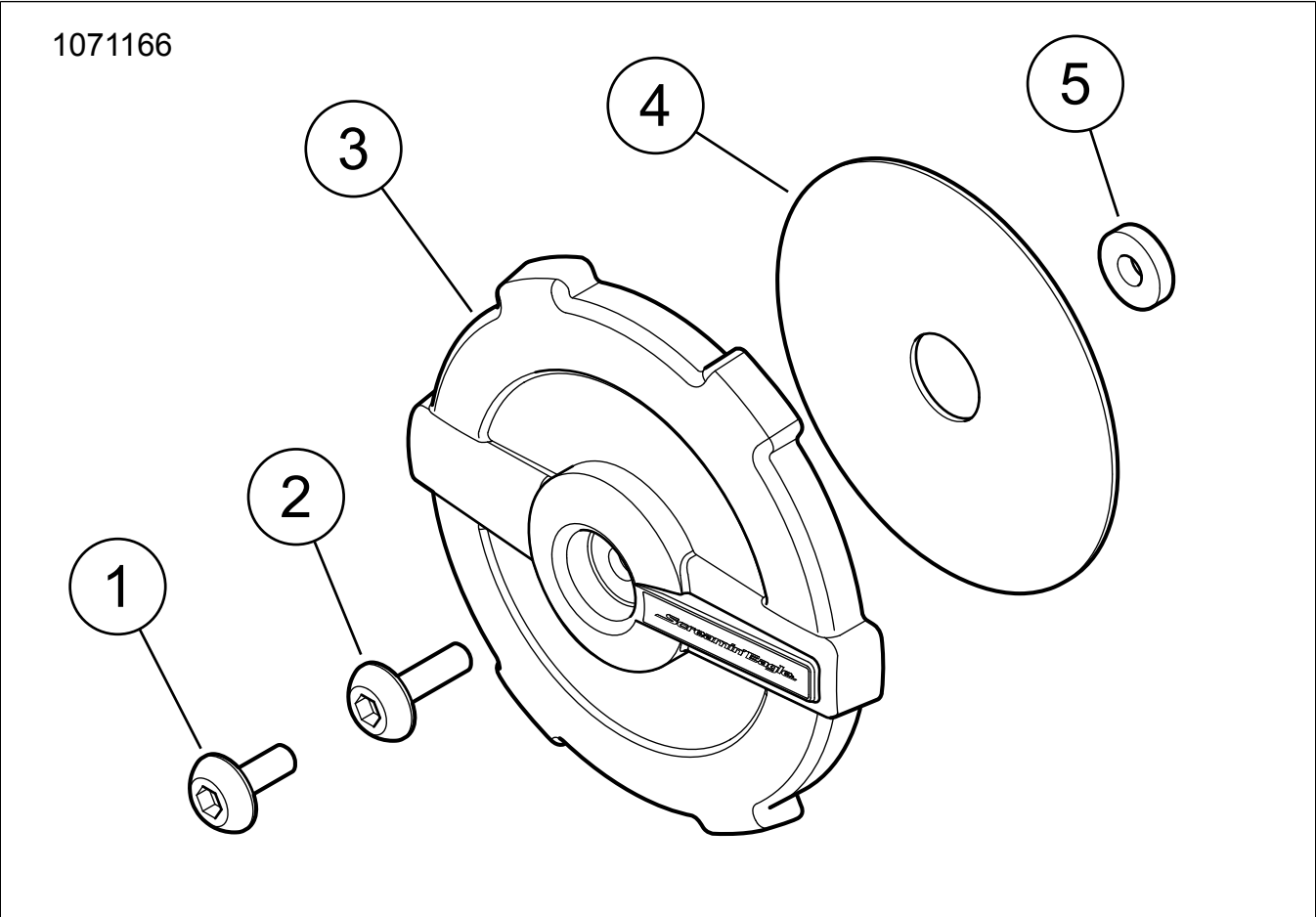
Figure 1. Air Cleaner Trim Kit
