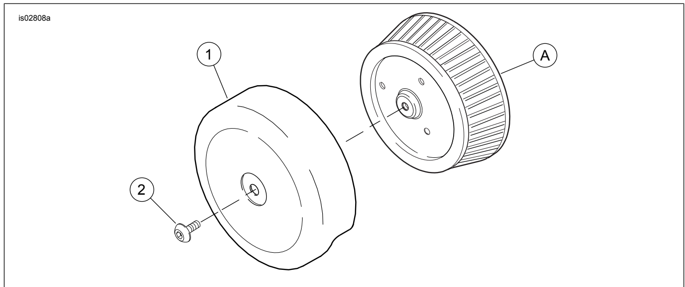
Figure 1. Service Parts: Air Cleaner Cover
