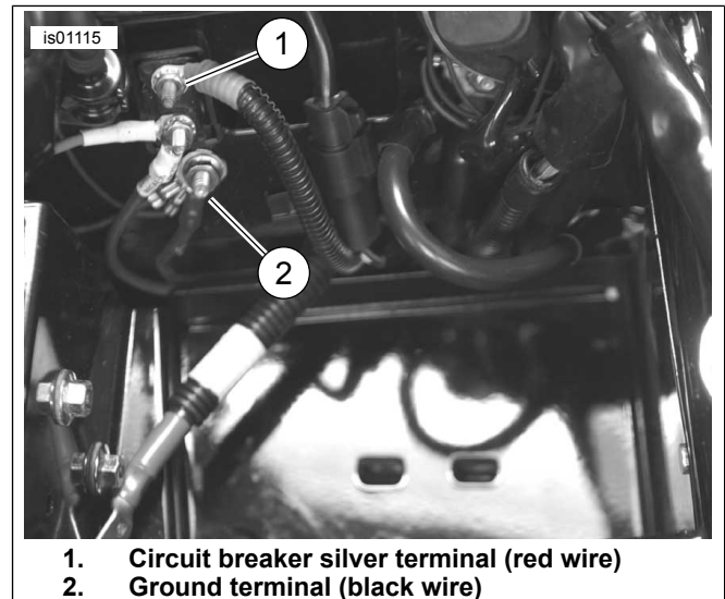
Figure 5. Connections (with battery removed) - 2003 or Earlier Touring Models (2003 FLHTCU shown)
