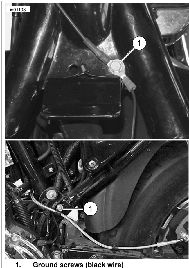
Figure 4. Ground Connections (Sportster Models)
