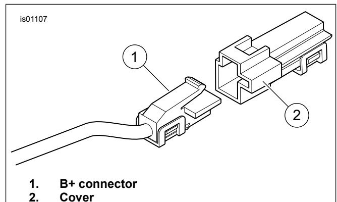
Figure 20. B+ Connector
