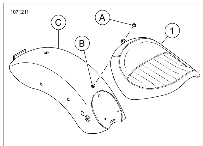
Figure 1. Service Parts: Single post mount
