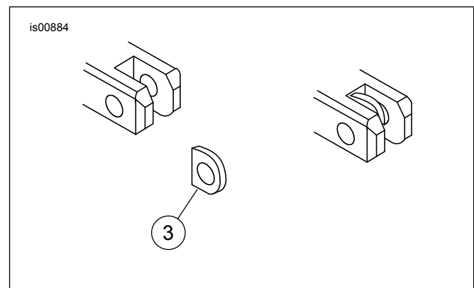
Figure 2. Footpeg Spring Washer Installation
