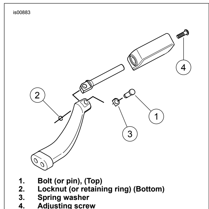
Figure 1. Footpeg Removal/Installation
