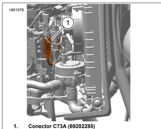
Figura 2. Conector C73A
