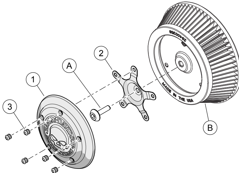
Figure 1. Kit Contents: Air Cleaner Cover
