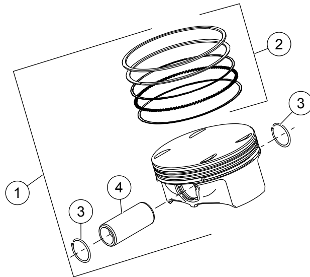
Figura 4. Pistuni u Flywheel tal-131 Screamin' Eagle Crate Engine
