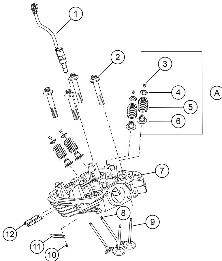
Figura 3. Cylinder Heads u Valvoli tal-131 Screamin' Eagle Crate Engine
