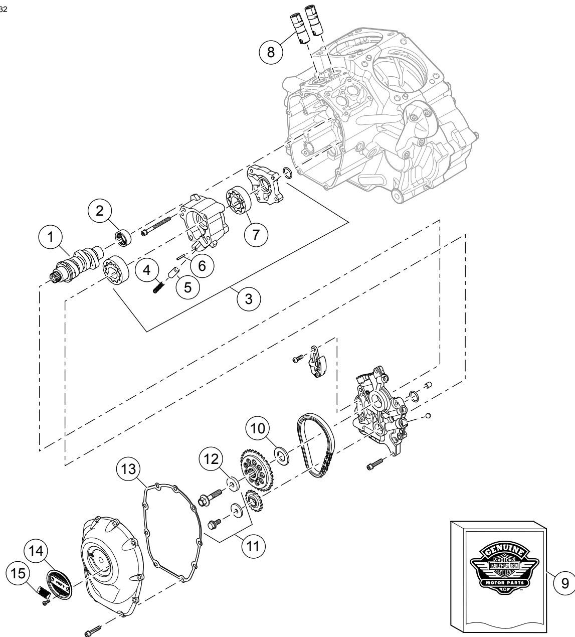
Figura 5. Kopertura tal-Kamxaft u Kamxafts tal-131 Screamin' Eagle Crate Engine
