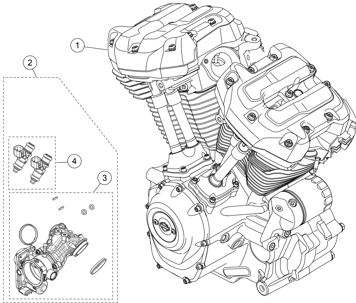
Figura 1. Assemblaġġ tal-Magna, Screamin' Eagle 131 Crate Engine Kompluta
