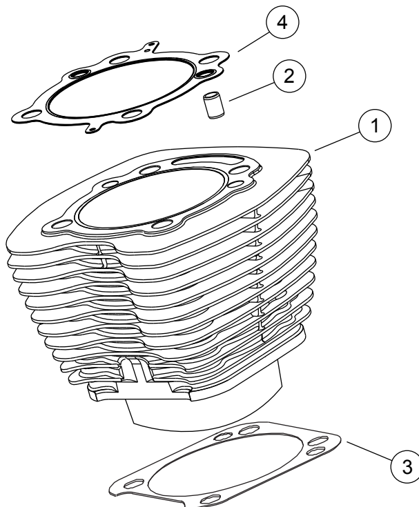
Figura 2. Ċilindri tal-131 Screamin' Eagle Crate Engine
