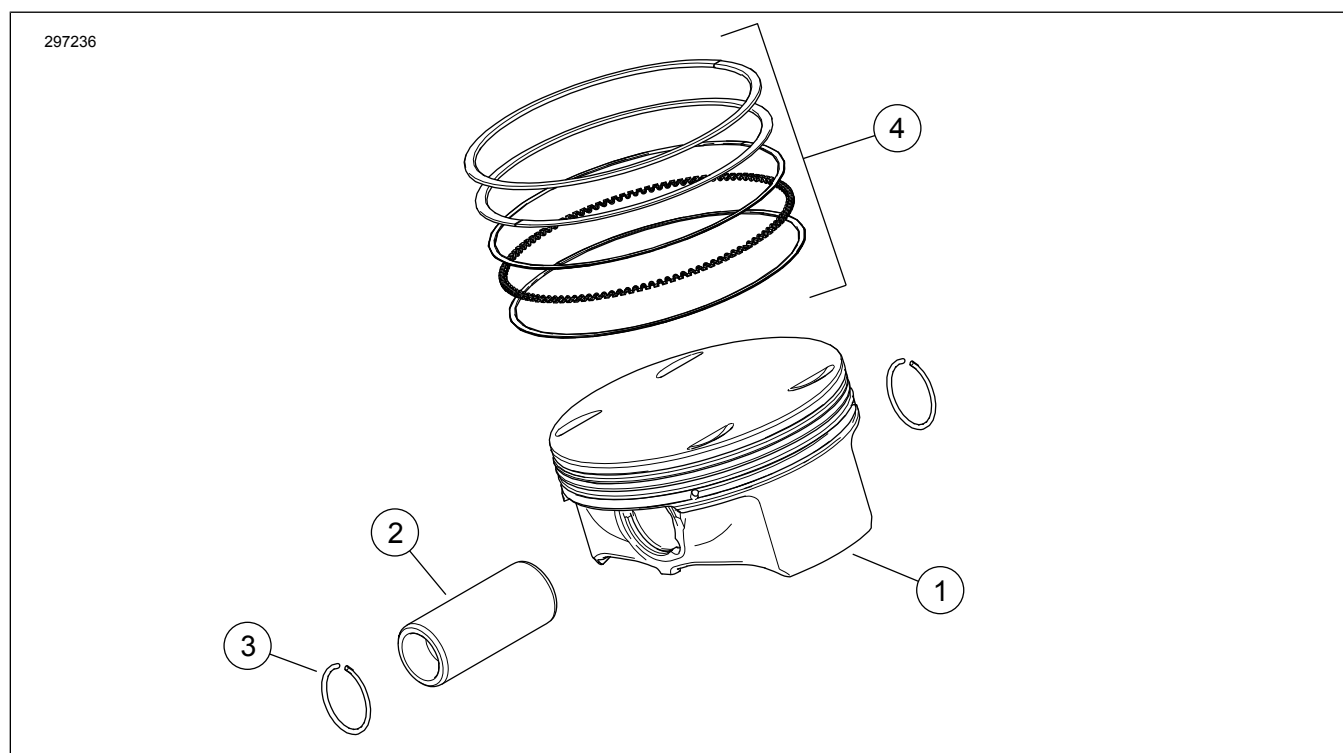
Figura 1. Parts tas-servizz: Kits tal-Pistun Screamin' Eagle Big Bore 128/131
