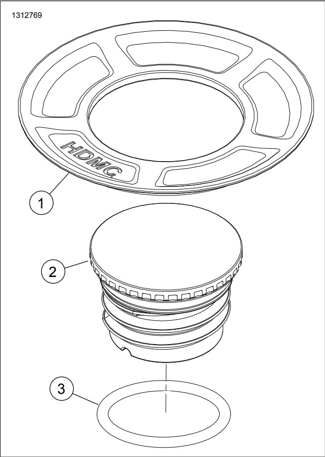
Figure 2. Service Parts: Flush-Mount Gas Cap Kit
