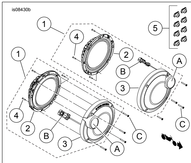
Figur 2. Servicedelar, BOOM! Audio Stage II bakre högtalarsats
