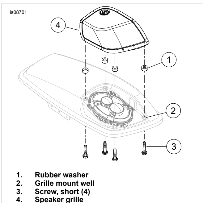
Figure 2. Grille Installation
