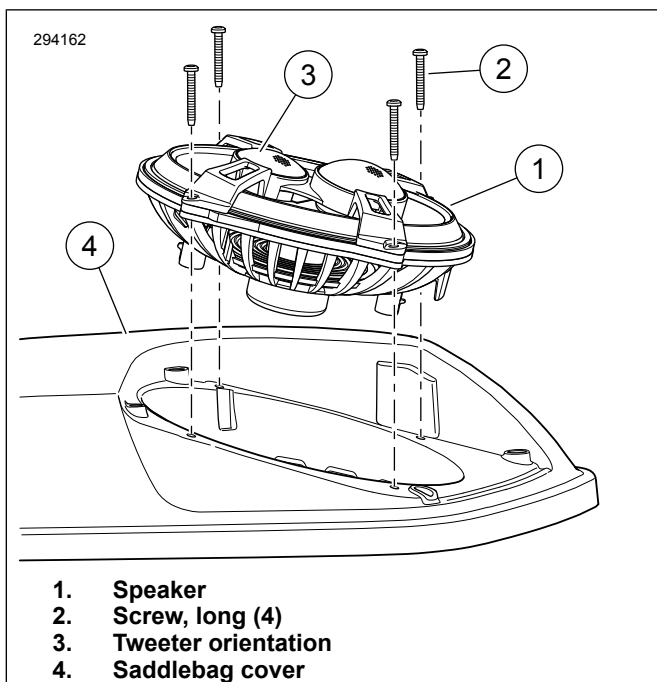
Figure 1. Speaker Orientation
