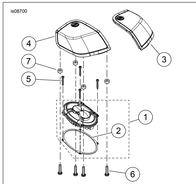
Figura 3. Parts tas-Service, Kit tal-Ispiker tas-Saddlebag Boom! Audio Stage II
