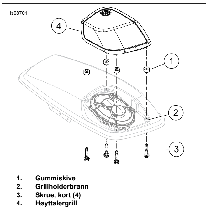
Figur 2. Grillmontering
