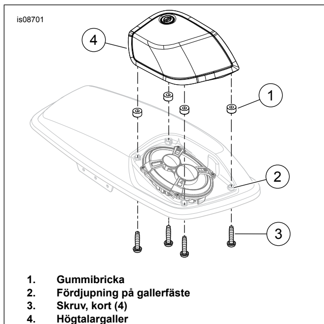
Figur 2. Gallermontering
