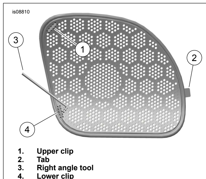
Figure 1. Remove Speaker Grille
