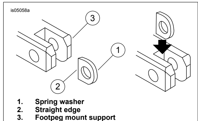
Figure 1. Spring Washer Installation
