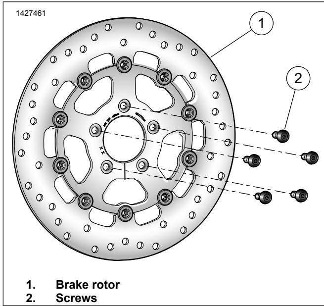
Figure 1. Service Parts: Front Brake Rotor (Disc) Kits
