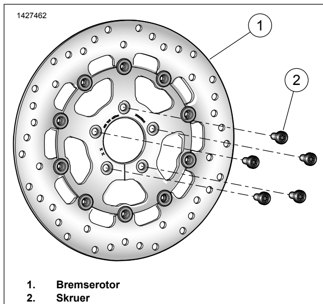
Figur 1. Servicedeler: Sett for bakre bremserotor
