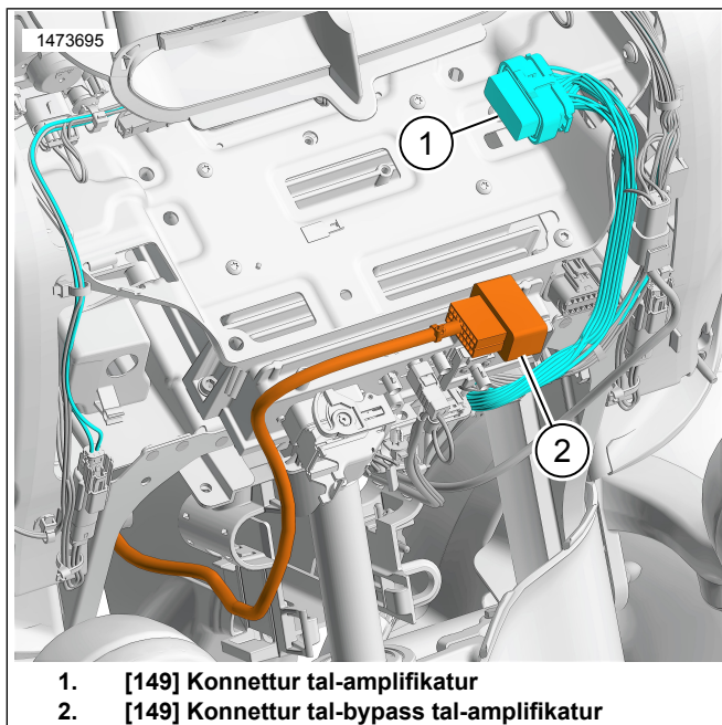
Figura 2. Jidher Fairing Immuntat fuq Furketta, Fairing Fiss huwa Simili
