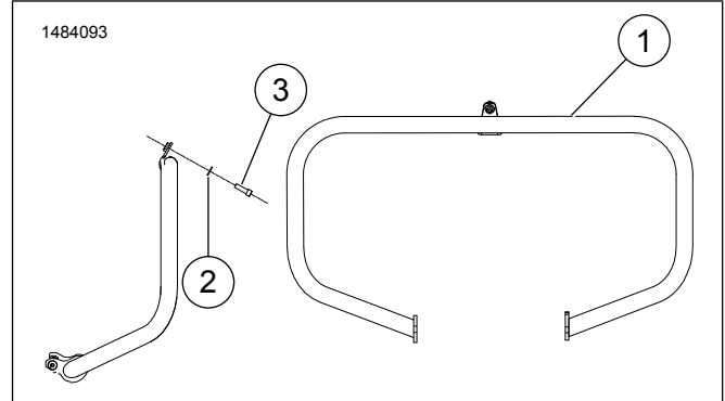
Figure 1. Service Parts: Engine Guard Kit
