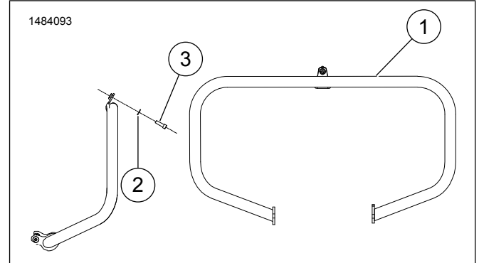
Figura 1. Parts tas-Service: Kit tal-lqugħ tal-Magna
