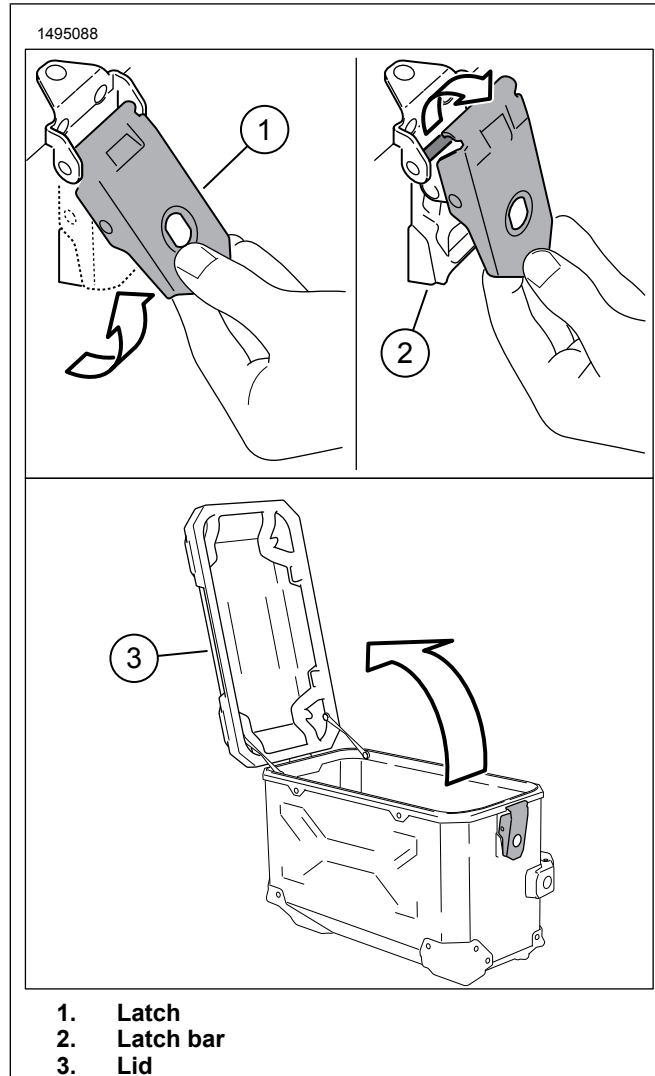
Figure 2. Opening Lid
