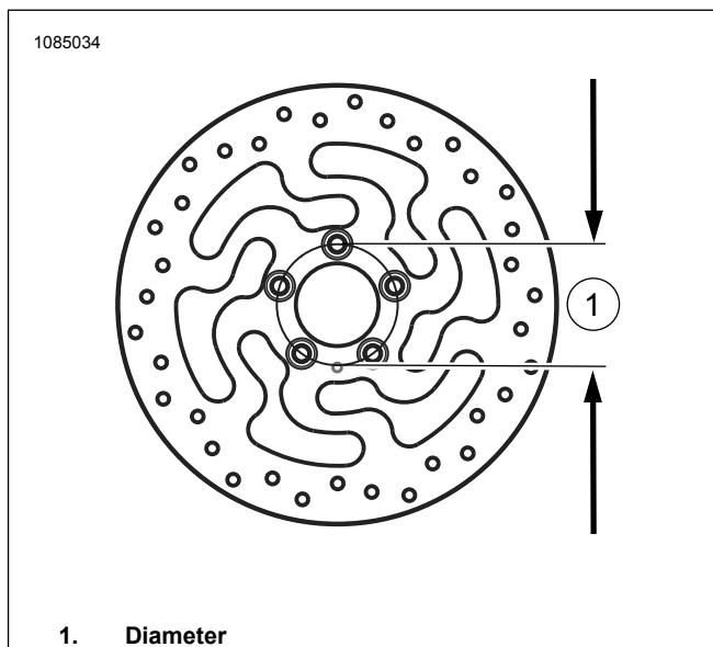
Figur 4. Diameter for skivemonteringshull
