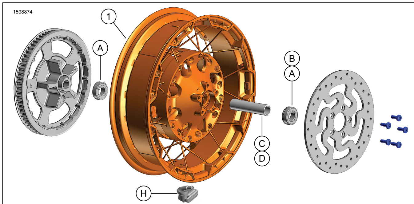
Figur 2. Bakhjulsett
