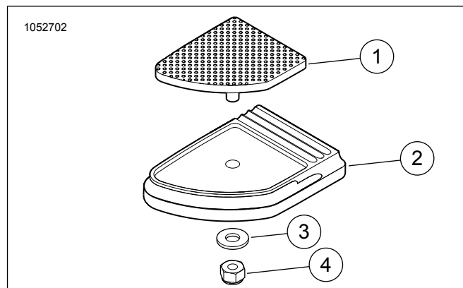
Figure 1. Service Parts: Small Brake Pedal Pad Kit
