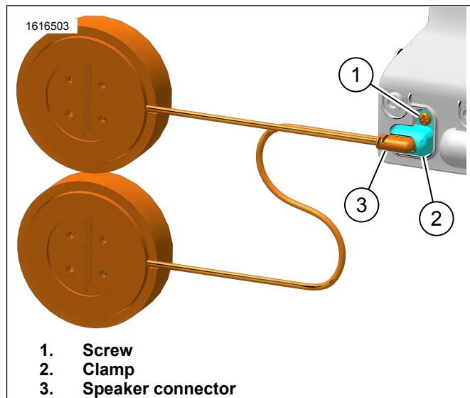
Figure 3. Speaker Assembled
