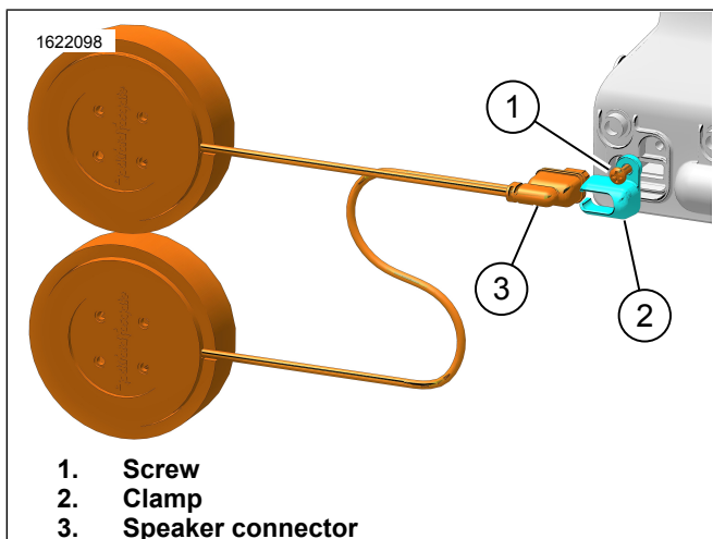
Figure 2. Disassembly
