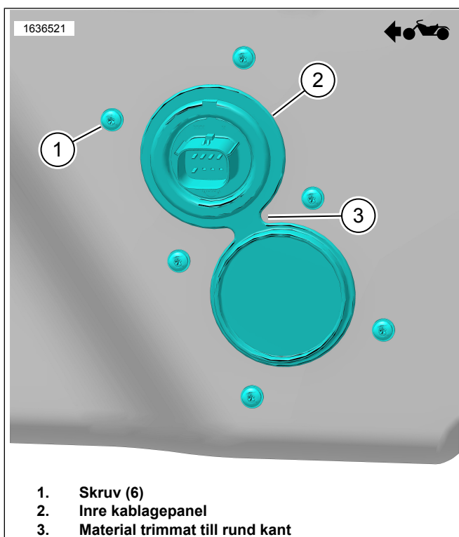
Figur 7. Inre kablagepanel
