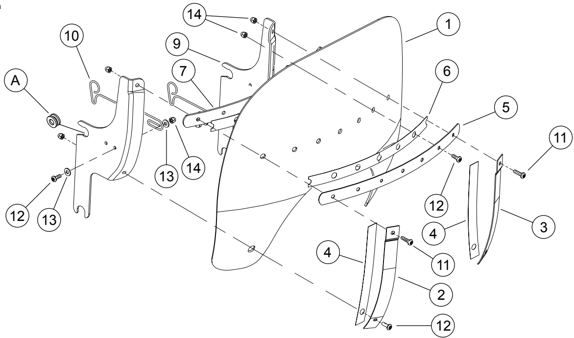
Figure 2. Kit Contents: Wind Deflector (Typical)
