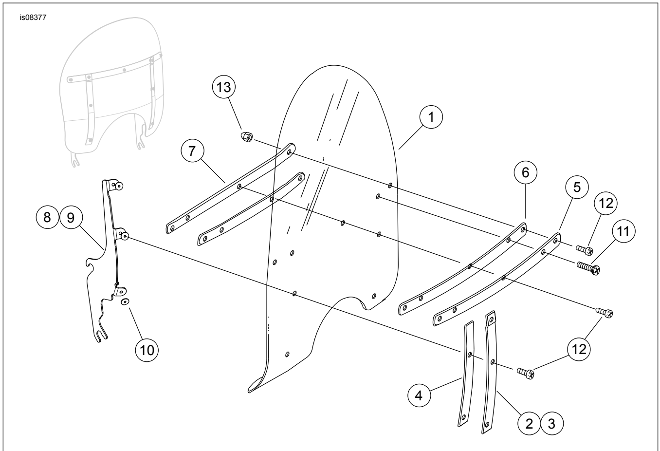
Figure 1. Kit Contents: Windshield (Typical)
