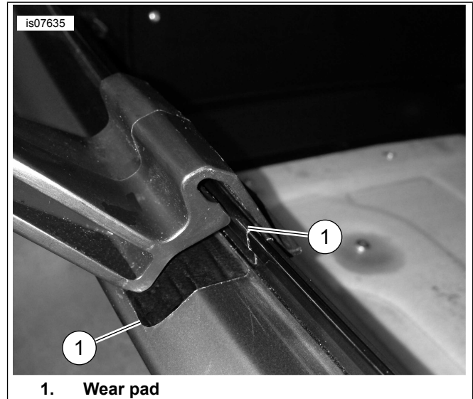
Figure 1. Install Wear Pad on Tour-Pak
