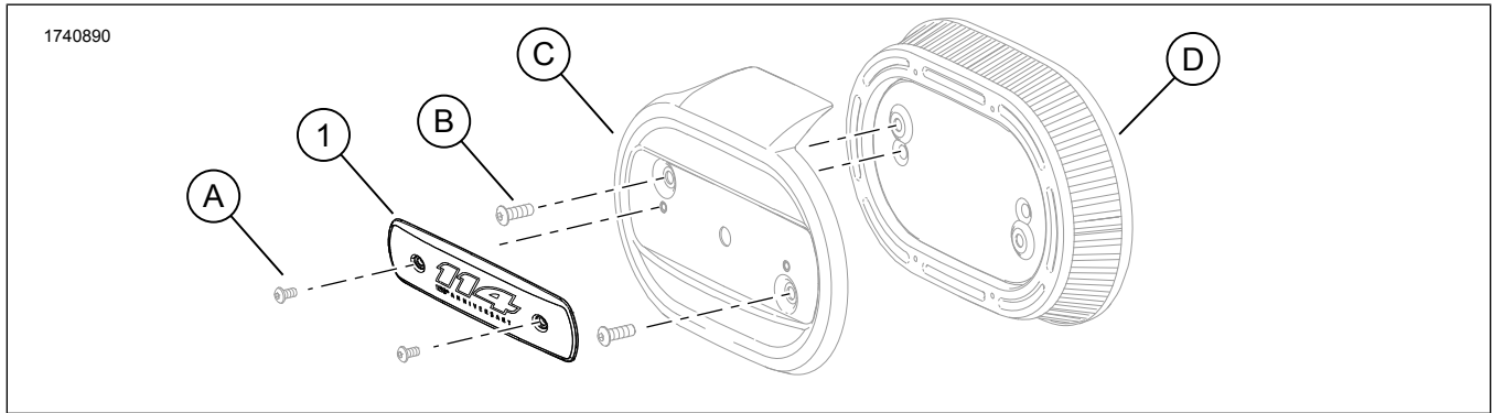
Figure 1. Kit Contents: 120th Anniversary Air Cleaner Cover Medallion
