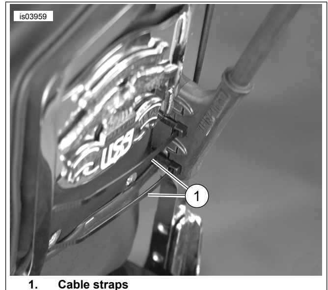
Figure 2. Interior View of Installed Flag Mast
