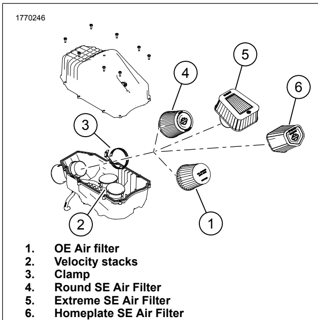
Figure 1. Air Box Cover (Typical)
