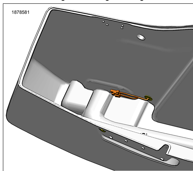
Figur 7. Jumper Harness Routing (hvis installeret)
