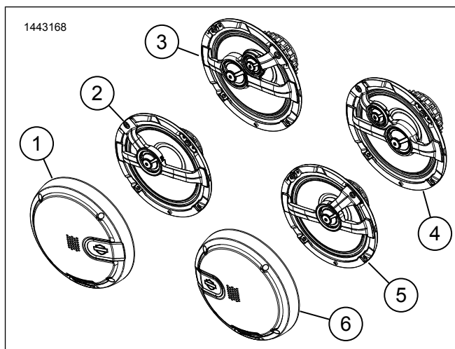
Figura 4. Piese de schimb, Kit difuzor spate BOOM! Audio 6.5
